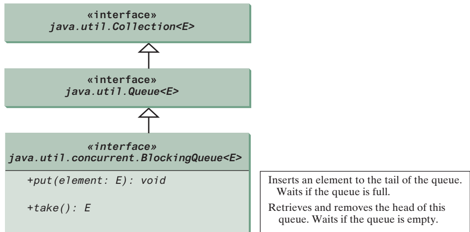
FIGURE 32.20 BlockingQueue is a subinterface of Queue .
