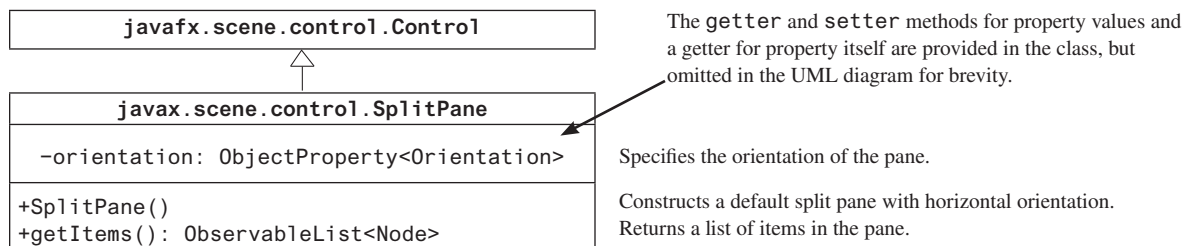
FIGURE 31.25 SplitPane provides methods to specify the properties of a split pane and for manipulating the components in a split pane.
