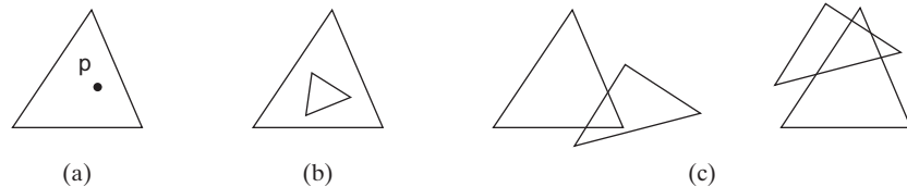
FIGURE 10.22 (a) A point is inside the triangle. (b) A triangle is inside another triangle. (c) A triangle overlaps another triangle.
