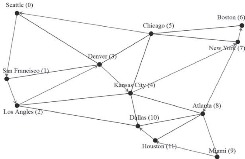
FIGURE 28.13 A DFS search starts from Chicago. Source: © Mozilla Firefox.
