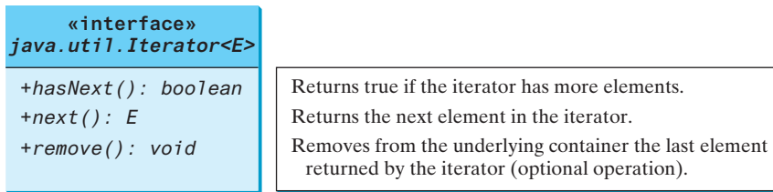
FIGURE 25.17 The Iterator interface defines a uniform way of traversing the elements in a container.
