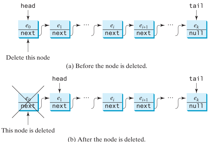
FIGURE 24.15 The first node is deleted from the list.
