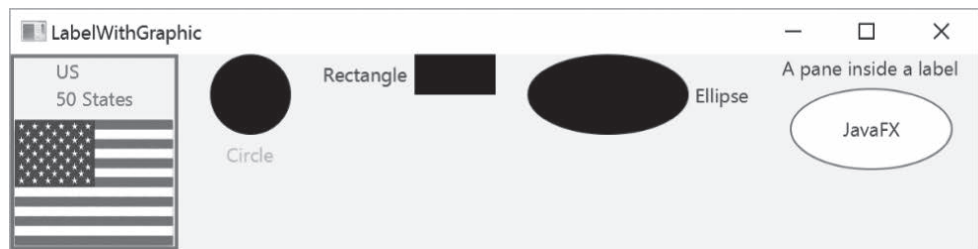
FIGURE 16.4 The program displays labels with texts and nodes. Source: booka/Fotolia.
